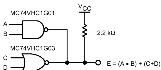
Figure 7. Complex Boolean Functions
